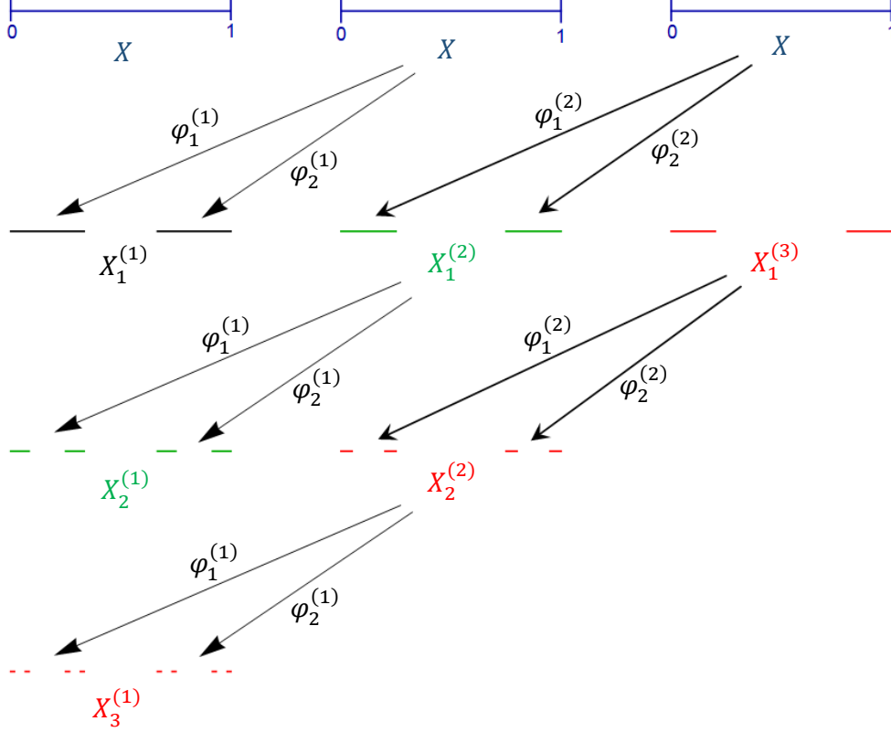
FIGURE 1. Table illustrating Example 2.3 with a_1 = \frac{1}{3} , a_2 = \frac{1}{4} , and a_3 = \frac{1}{5} . Note that sets in each column decrease down to the corresponding limit set, i.e., for each j \in \mathbb{N} we have \bigcap_{k=1}^{\infty} X_k^{(j)} = J^{(j)} . Also, note that diagonally adjacent sets X_{k+1}^{(j)} and X_k^{(j+1)} are related by the invariance condition (2.1) in Remark 2.2.
