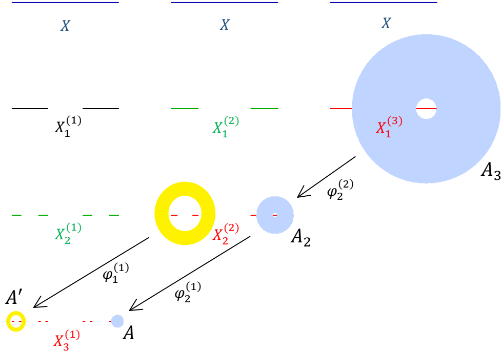
FIGURE 3. Illustration of the proof of Theorem 1.1 using the system of Example 2.3. Note that A and A_2 = (\varphi_2^{(1)})^{-1}(A) are both of Case (II) type, whereas A' is of Case (II) type, but (\varphi_1^{(1)})^{-1}(A') is of Case (I) type.
