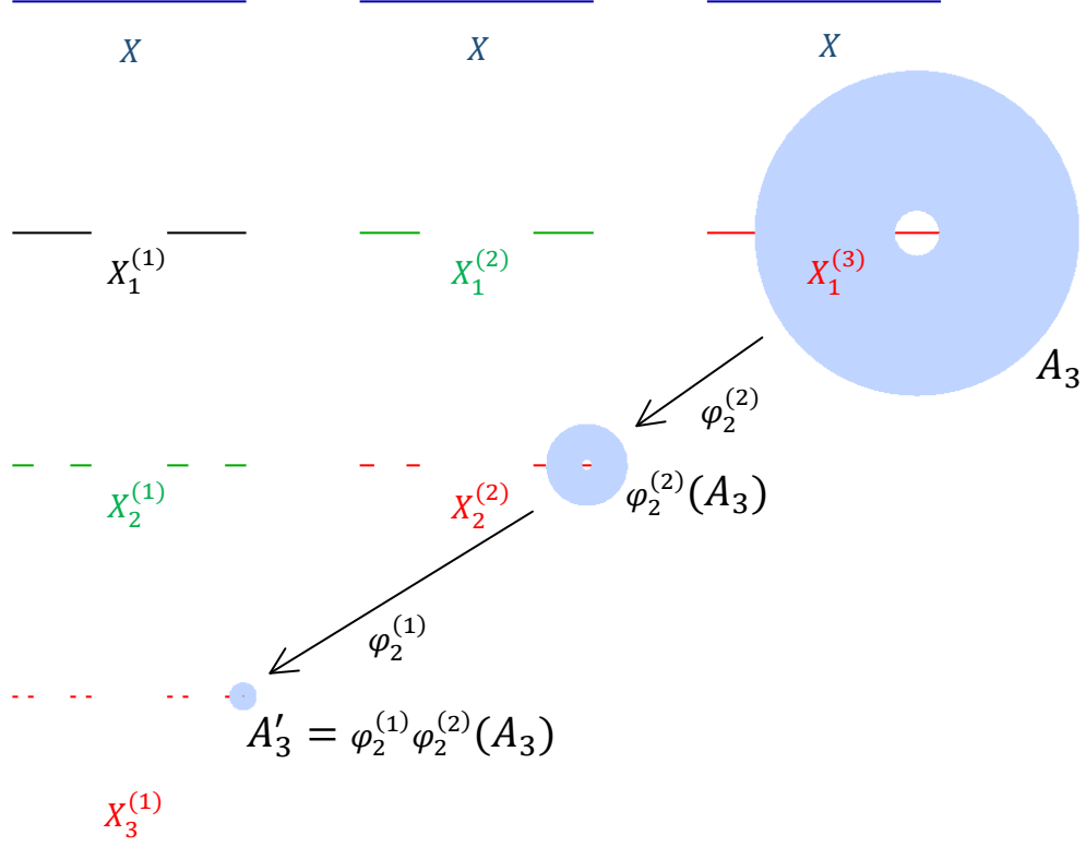
FIGURE 4. Table illustrating the proof of Theorem 1.1 using the system of Example 2.3.
