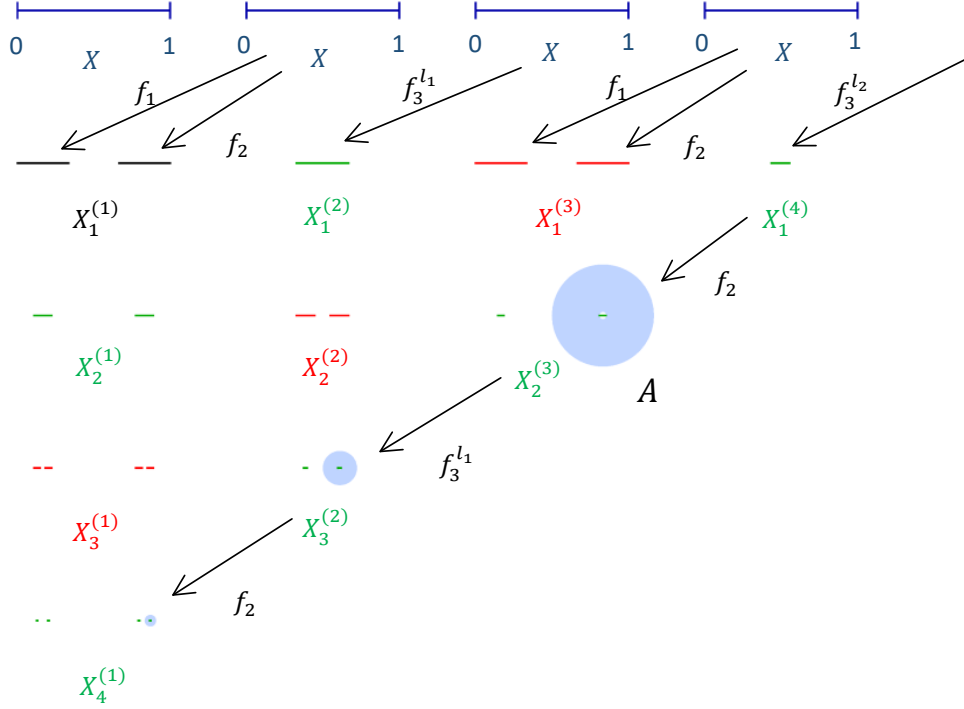
FIGURE 2. Table illustrating \tilde{\Phi} in Example 5.2, where l_1 = 1 and l_2 = 2 .
